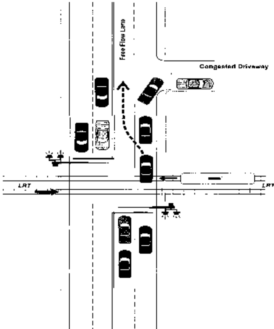
Figure 8. Motor vehicle escape channelization.
