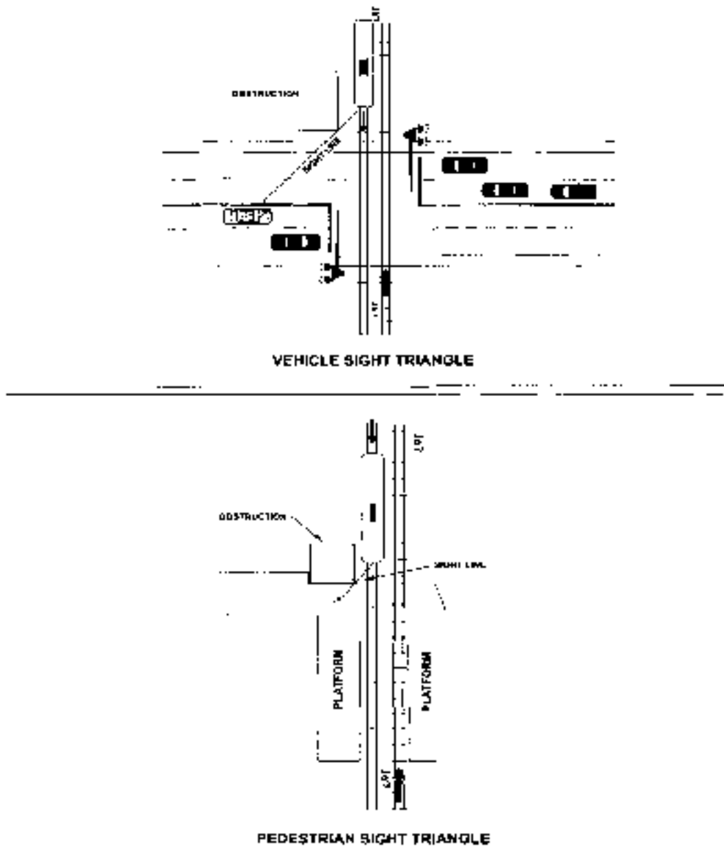
Figure 7. Sight distance.
