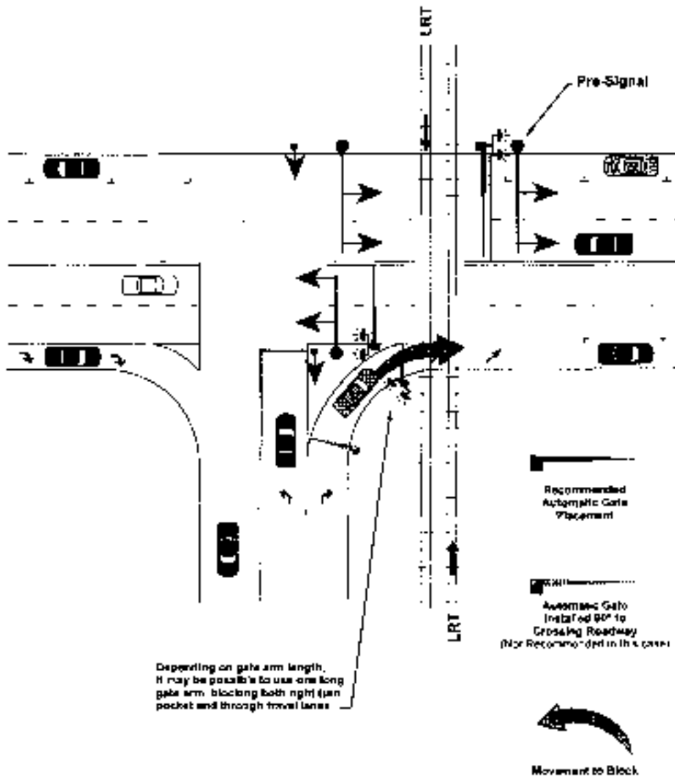
Figure 25. Right-turn automatic gate placement.
