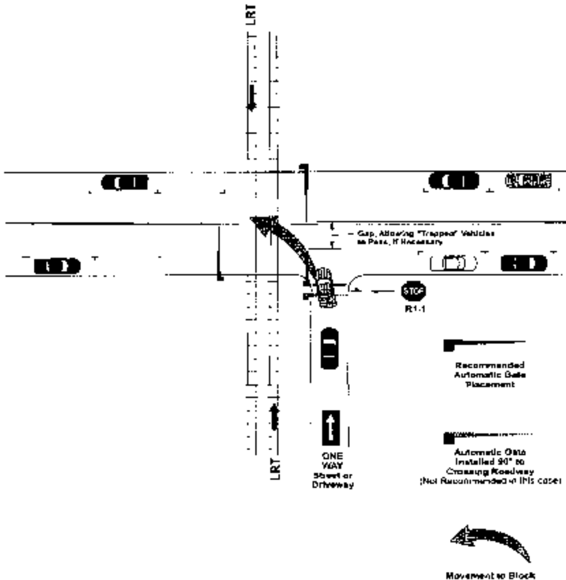
Figure 23. Left-turn automatic gate placement.
