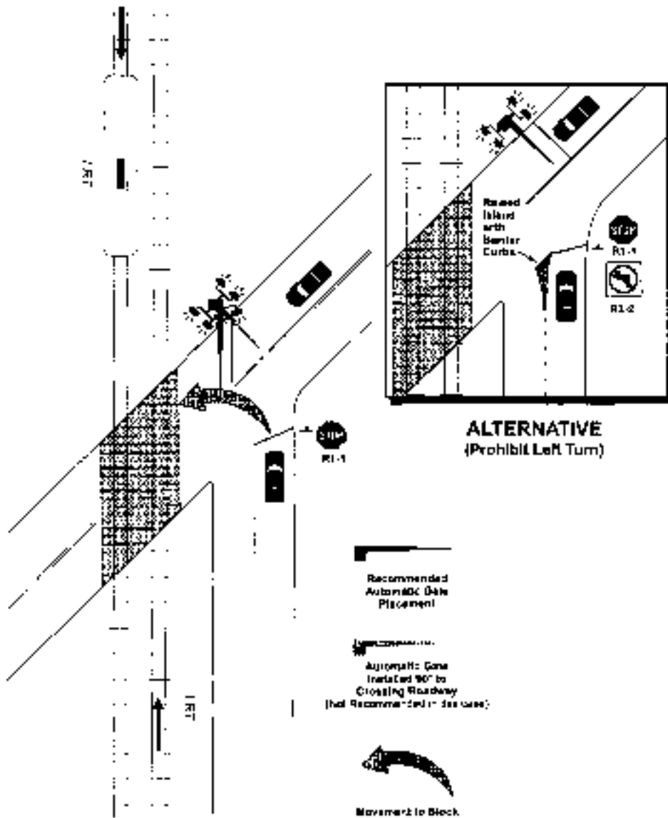
Figure 22. Automatic gate placement for turning traffic.
